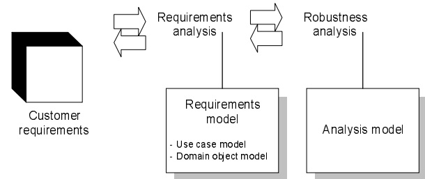
Figure 2: Analysis phase of the OOSE life cycle.
