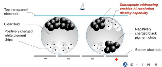
Cross-Section of Electronic-Ink Microcapsules
