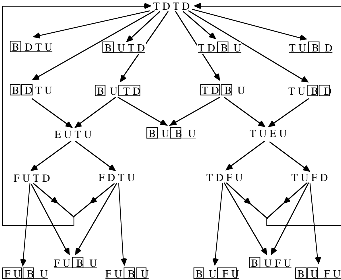
Figure 5.2. The low level transition system for Dinner. States with boxes are invisible and each box represents the range of a mark; for instance, \boxed{B} U \boxed{T} D represents ((*(up\ down\ down\ T)|(down^- D))* (TID)) \setminus up \setminus down . Underlined states correspond to deadlock states. All transitions are labelled by \tau .
