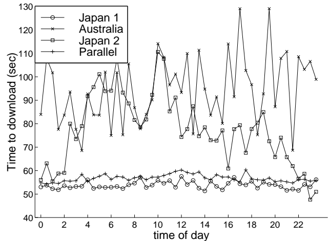
(a) S = 256 KBytes, B = 20 , M = 3 .
