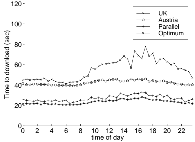
Fig. 6. Dynamic parallel-access . S = 5 Mbytes, B = 40 , M = 2 .
