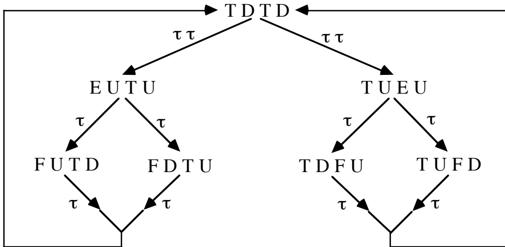
Figure 5.3. The high level system for Dinner. The two transactions are labelled by \tau\tau .
