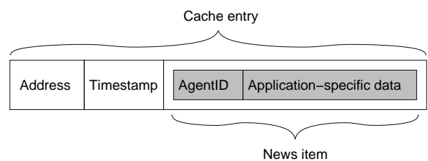
Figure 2. The format of news items and cache entries.
