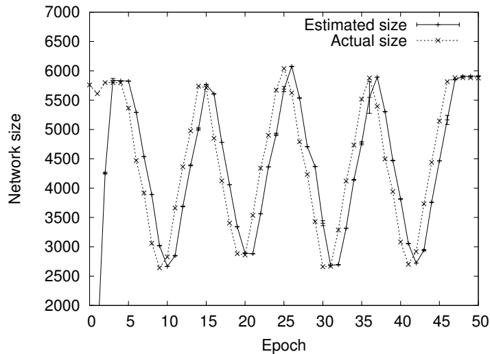
Figure 18: The estimated size (as provided by COUNT ) and the actual size of a network oscillating between 2500 and 6000 nodes (approximately). Standard deviation of estimated size is displayed using vertical bars.
